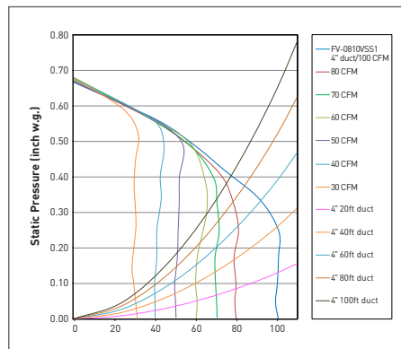
FV-0810VSSL1 80 or 100 CFM 4" Oval Duct
